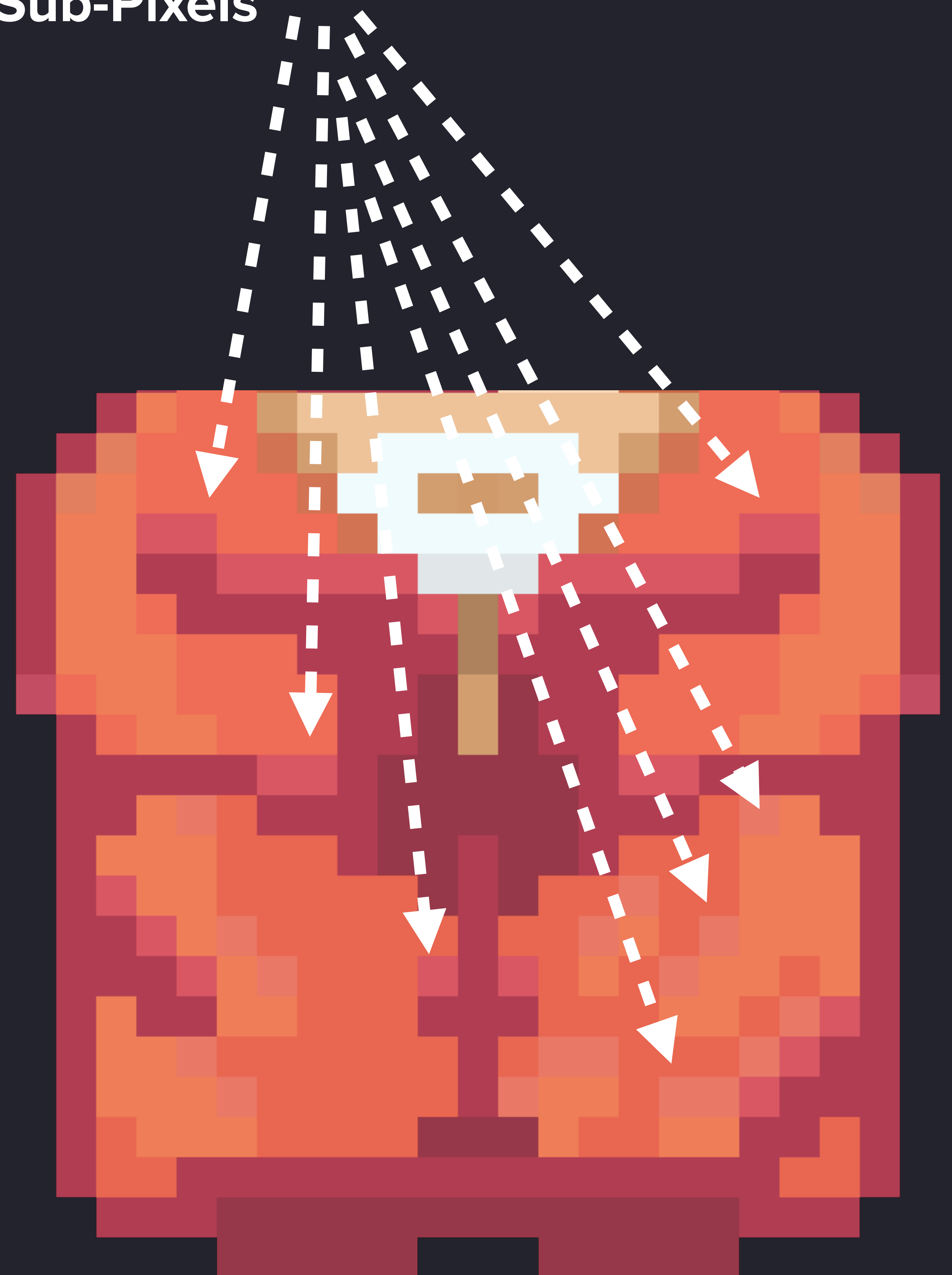
Sub-Pixel Animation
